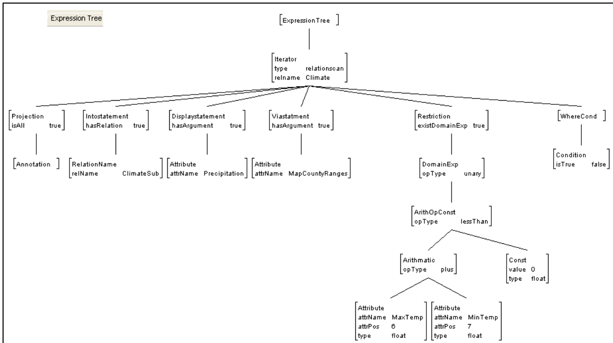
Figure 5.3 (b) Expression tree (graphical view)
